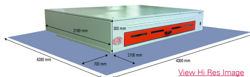
Floor Plan
