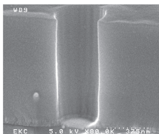
After Clean with DuPont™ PlasmaSolv® Post-Etch Residue Remover
